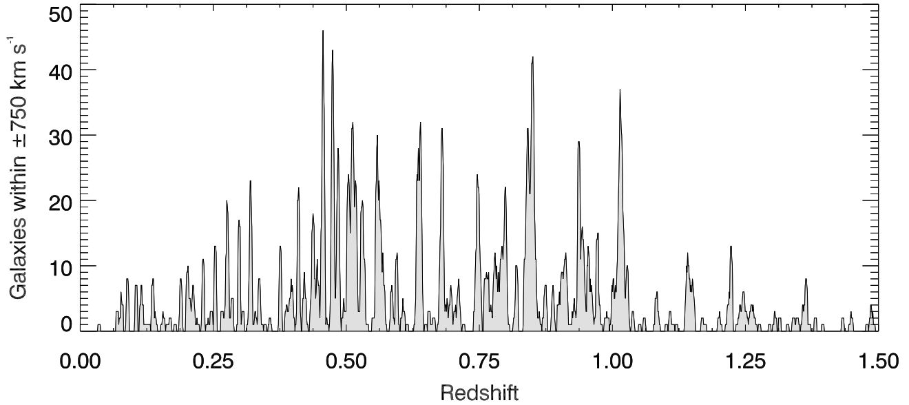
FIG. 16.— Redshift distribution of galaxies with secure measurements in the present sample. The raw marginal distribution was smoothed with a moving top hat kernel tuned to highlight structures similar in velocity dispersion to those noted in the HDF (Cohen et al. 2000). The ordinate represents the number of galaxies within \pm 750 \text{ km s}^{-1} at any given redshift. Several galaxies at high redshift are not shown.
